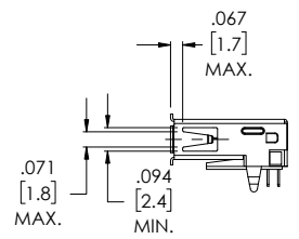
RECOMMENDED SIDE NOTCH SIZE FOR MATING A FEMALE CONNECTOR
