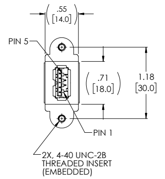
"J1" USB 3.0 SERIES "A" RECEPTACLE PANEL MOUNT CONTACTS: 30 μINCHES GOLD PLATING
