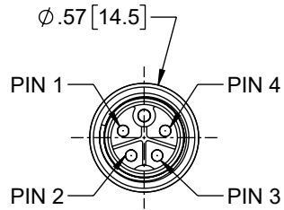
P1 M12 MALE CONNECTOR 4 POSITION L-CODED
