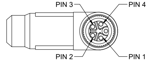
P2 M12 FEMALE RIGHT ANGLE CONNECTOR 4 POSITION L-CODED
