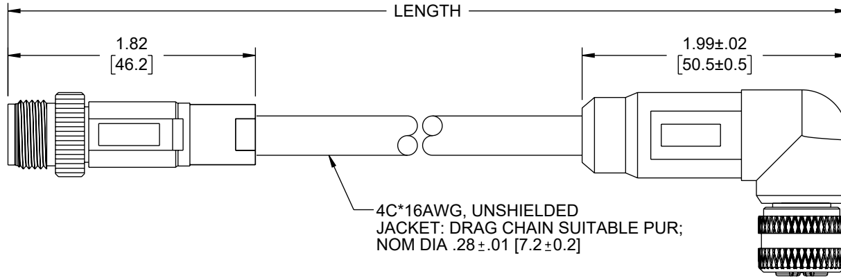
P1 M12 MALE CONNECTOR 4 POSITION L-CODED
