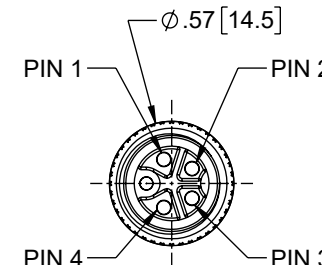
P2 M12 FEMALE CONNECTOR 4 POSITION L-CODED
