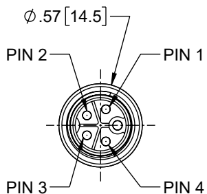
P1 M12 MALE CONNECTOR 4 POSITION L-CODED
