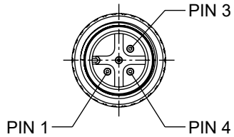
P1 M12 FEMALE CONNECTOR 3 POSITION A-CODED
