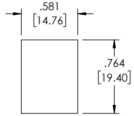
RECOMMENDED PANEL OPENING
