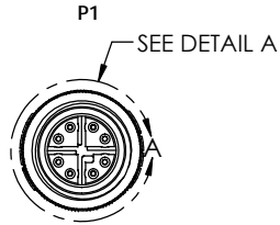
M12 SHIELD MALE 8 POSITION X-CODED
