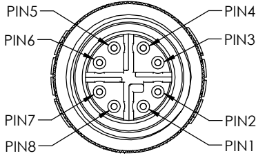
DETAIL A CONNECTOR PIN ASSIGNMENT
