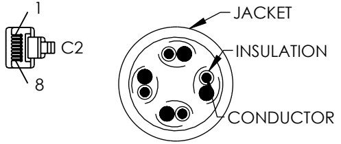
CABLE CROSS SECTION
