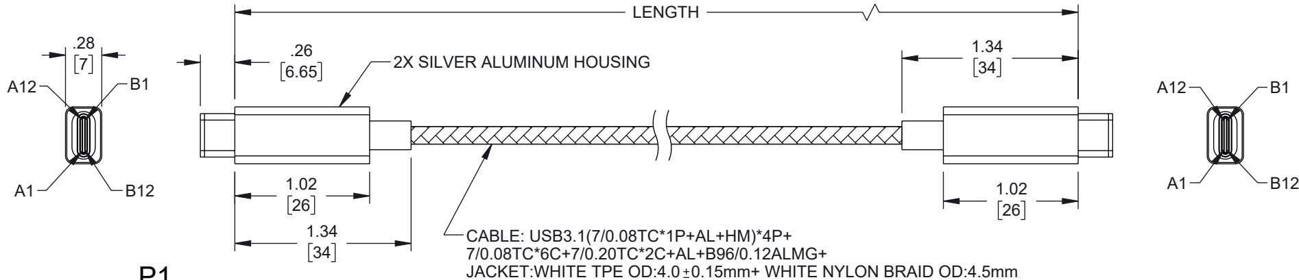
P2 USB 3.1 TYPE C MALE CONNECTOR W/ NICKEL PLATED CONTACTS
