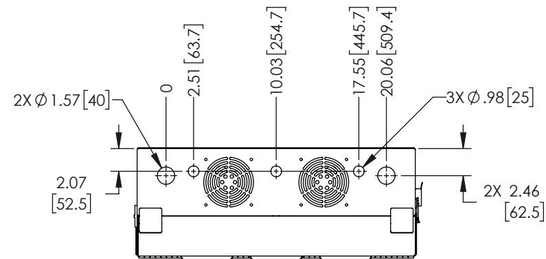
VIEW C-C
