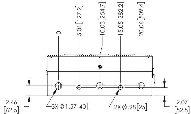
VIEW B-B
