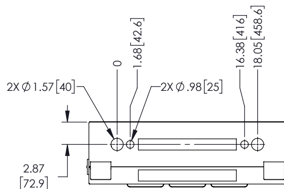
VIEW C-C
