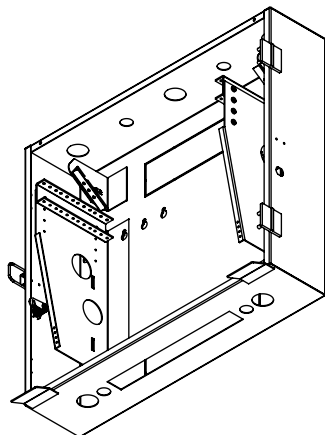
VIEW A-A POPULATED ENCLOSURE DOOR NOT SHOWN
