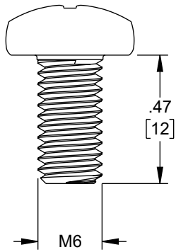
M6 ROUND HEAD SCREW
