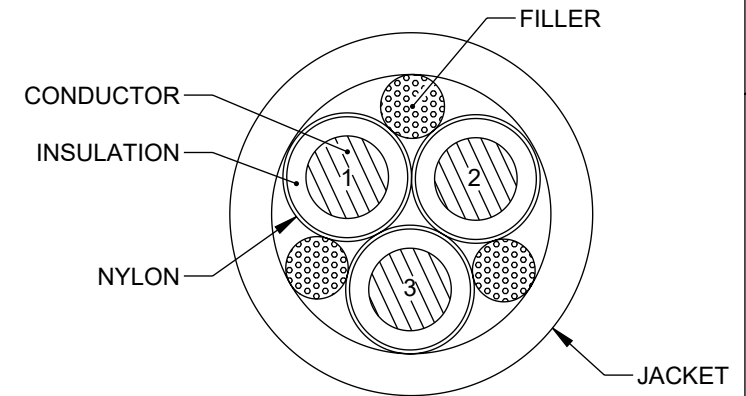
CROSS-SECTIONAL VIEW
