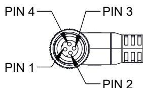
"P1" M12 SHIELDED MALE CONNECTOR 4 POSITION, D-CODED
