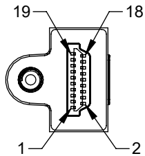
P1 HDMI AM 19P PIN: G/F SHELL: GOLD PLATED
