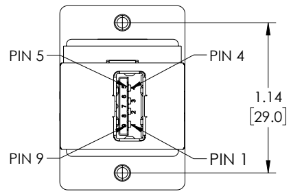
"J2" USB 3.0 TYPE "A" FEMALE CONNECTOR 30U" GOLD PLATED CONTACTS NICKEL PLATED SHELL
