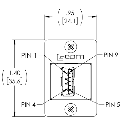
"J1" USB 3.0 TYPE "A" FEMALE CONNECTOR 30u" GOLD PLATED CONTACTS NICKEL PLATED SHELL
