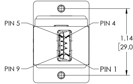
"J2" USB 3.0 TYPE "A" FEMALE CONNECTOR 30U" GOLD PLATED CONTACTS NICKEL PLATED SHELL
