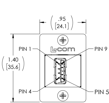
"J1" USB 3.0 TYPE "A" FEMALE CONNECTOR 30U" GOLD PLATED CONTACTS NICKEL PLATED SHELL
