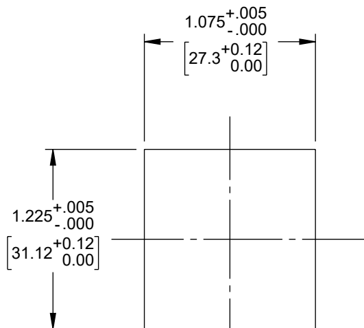
PANEL DETAIL
