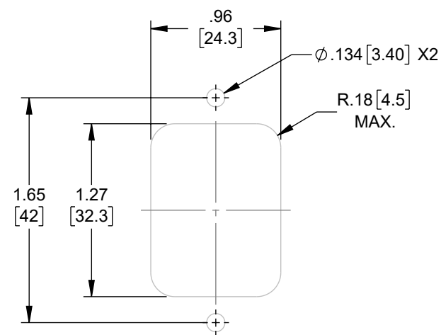
FIXING DETAILS
