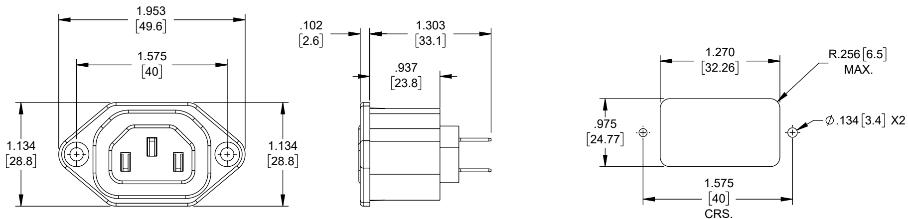
FIXING DETAILS
