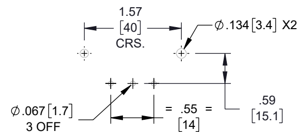
P.C.B. FIXING DETAILS
