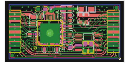
HDMI PCB
